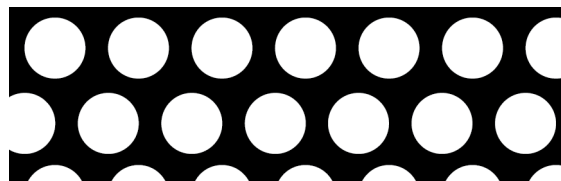
RV 8,0/11,0; a_o = 48,0\%
