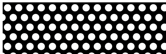
RV 3,0/5,0; a_o = 32,7\%
