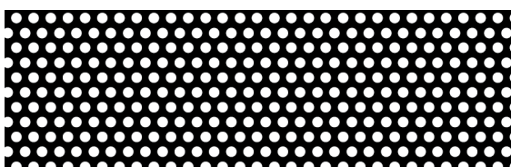
RV 1,5/2,4; a_o = 32,7\%
