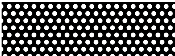
RV 2,0/3,5; a_o = 29,6\%
